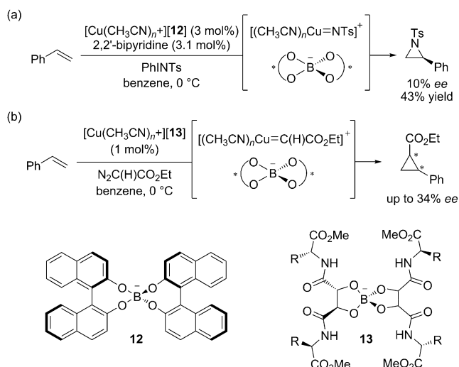
Scheme 6. Proof-of-concept studies using chiral borate anions.
