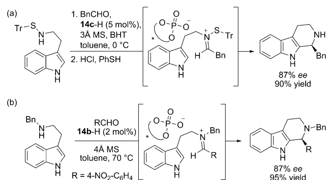
Scheme 12. Phosphoric acid-catalyzed Pictet–Spengler reaction proceeding via a) sulfonyliminium ions or b) dialkyl iminium ions.
