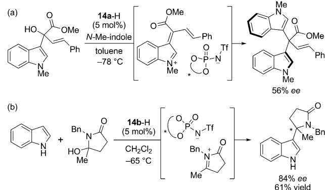
Scheme 21. N -triflylphosphoramidate-catalyzed nucleophilic addition to a) N -alkylindolium and b) N -acyliminium ions.
