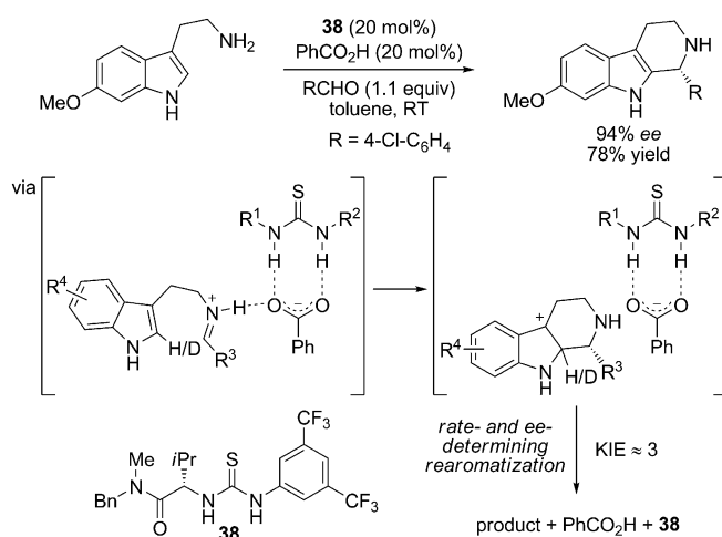
Scheme 36. Thiourea-catalyzed enantioselective Pictet–Spengler reaction with rate-determining rearomatization.
