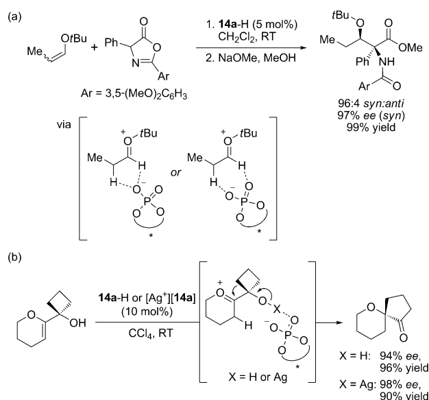
Scheme 16. a) Aldol-type reaction and b) semipinacol rearrangement of oxocarbenium ions formed in situ by the protonation of vinyl ethers.
