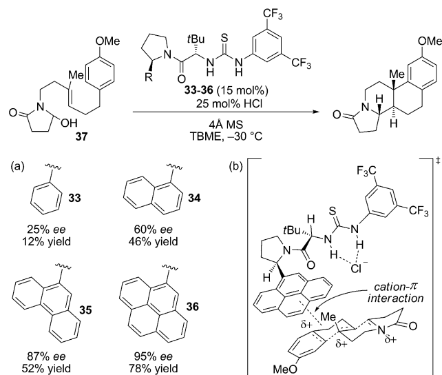
Scheme 33. a) Effect of thiourea catalyst aromatic group on the efficiency and enantioselectivity of the bicyclization of hydroxylactam 37 and b) the proposed stabilizing cation-π interaction in the dominant transition state.
