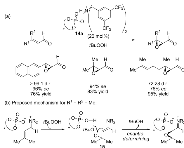
Scheme 9. a) Scope and b) mechanism for the epoxidation of enals catalyzed by chiral secondary ammonium-phosphate salts.
