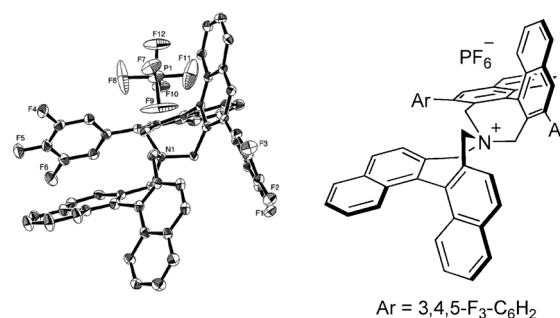
Figure 7. X-ray crystal structure of N -spiro binaphthyl catalyst ( 2 )· PF_6^- (adapted from reference [28]).
