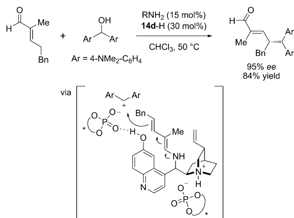
Scheme 14. Cooperative dienamine and ion-pairing catalysis for the δ-alkylation of α-branched enals.
