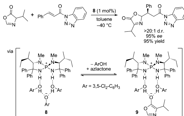
Scheme 3. Tetraaminophosphonium salt 8 as a supramolecular chiral organic base catalyst for conjugate additions to acylbenzotriazoles.
