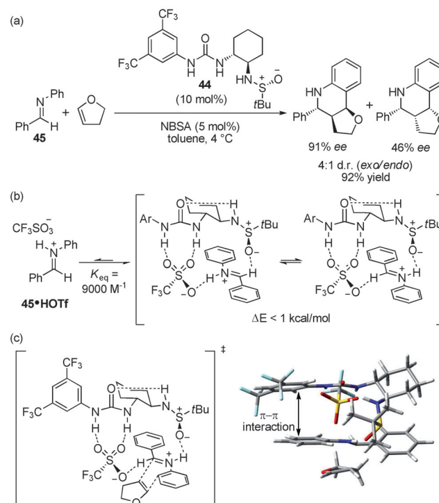
Scheme 42. a) Urea/strong Brønsted acid co-catalyzed enantioselective Povarov reaction (NBSA = o -nitrobenzenesulfonic acid). b, c) Energy- and geometry-minimized structures of b) the ground state catalyst-substrate interactions (Ar = 3,5-(CF 3 ) 2 -C 6 H 3 ) and c) the cycloaddition transition structure leading to the major enantiomer of product at the B3LYP/6-31G(d) level of theory.
