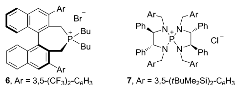
Figure 9. Representative chiral phosphonium phase-transfer catalyst structures.
