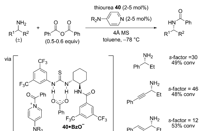
Scheme 38. Acylative kinetic resolution of primary amines by an anion-binding approach to nucleophilic catalysis.
