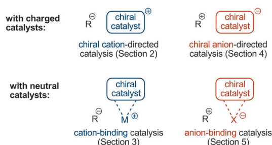
Figure 1. Types of asymmetric ion-pairing catalysis.
