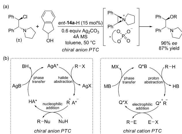
Scheme 17. a) Desymmetrization of meso -aziridinium ions by chiral phosphate-directed PTC and b) the proposed catalytic cycle for this application of chiral anion PTC compared to chiral cation PTC (X = halide, B = basic anion, A* = chiral anion, Q* = chiral cation, M = alkali metal).
