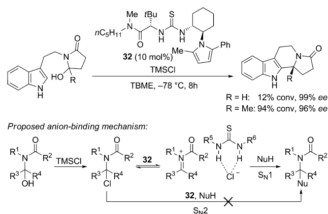
Scheme 31. Pictet–Spengler-type cyclization of hydroxylactams and the proposed anion-binding mechanism.
