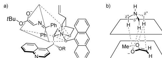
Figure 5. a) Tetrahedron stereoselectivity model for cinchona alkaloid-derived catalysts and the proposed enolate approach based on b) the optimal geometry for attractive R_3N^+-C-H \cdots X bonds in the [Me_3NH-CH_2COOMe] complex at the MP2/6-311++G** level of theory.
