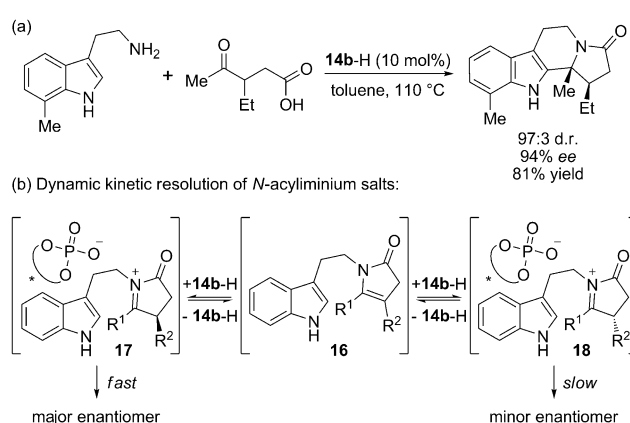
Scheme 10. a) Enantioselective phosphoric acid-catalyzed N -acyliminium ion cyclization cascade and b) the proposed mechanism.
