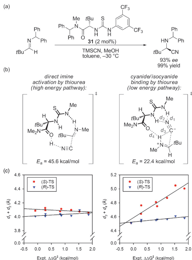
Scheme 28. a) Thiourea-catalyzed enantioselective Strecker reaction, b) potential activation mechanisms, and c) correlation of selected, calculated transition structure hydrogen-bond lengths with enantioselectivity for the hydrocyanation of N -benzhydryl pivaldimine for eight structurally distinct thiourea catalysts.
