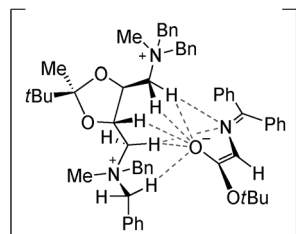
Figure 8. Optimized structure of a tartrate-derived diammonium catalyst ( 3 )·enolate ion pair at the B3LYP/6-31G(d) level of theory.
