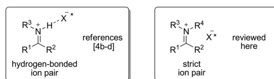
Figure 11. Types of ion-pairing interactions.
