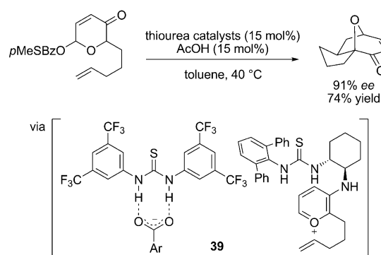
Scheme 37. Enantioselective oxidopyrylium-based [5+2] cycloaddition via anion-binding/enamine co-catalysis.
