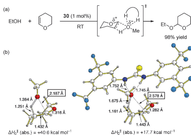
Scheme 27. a) Thiourea-catalyzed tetrahydropyranylation of alcohols by anion-binding and b) a comparison of transition structures for the uncatalyzed and thiourea-catalyzed addition of methanol to dihydropyran at the B3LYP/6-31G(d,p) level of theory (adapted from reference 105).
