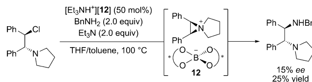
Scheme 7. Chiral borate anion-directed aziridinium opening reaction.
