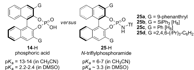
Figure 13. Acidity of phosphoric acid versus N -triflylphosphoramidate catalysts. [86,87]
