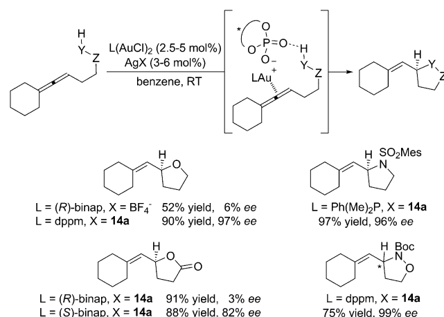
Scheme 20. Chiral phosphate-directed Au I -catalyzed enantioselective hydrofunctionalization of allenes.
