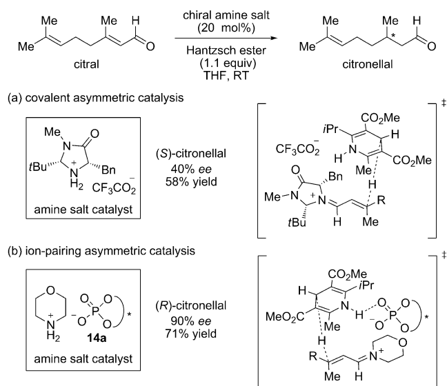
Scheme 8. Comparison of enantioselective transfer hydrogenations of enals via iminium catalysis by a) chiral ammonium- or b) chiral anion-based salts.
