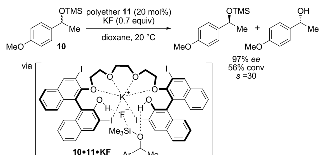
Scheme 5. Bis(hydroxy) polyether-catalyzed desilylative kinetic resolution of silyl-protected secondary alcohols.
